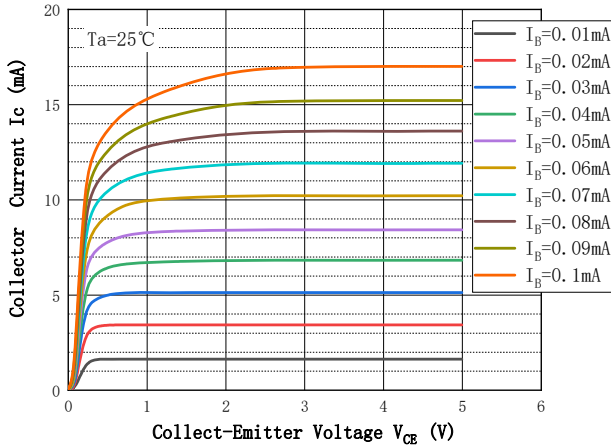
Fig.1-Static Characteristic
