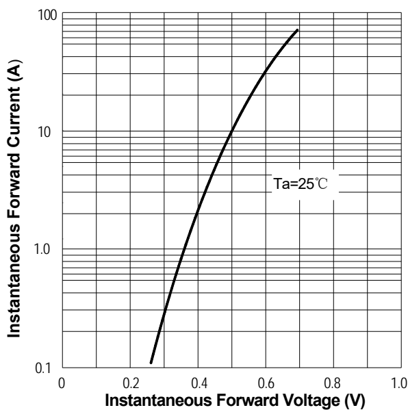
FIG.3: Forward Voltage
